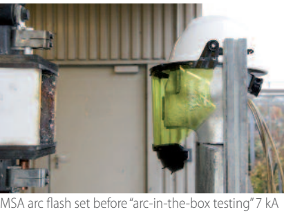
MSA arc flash set before "arc-in-the-box testing" 7 kA
